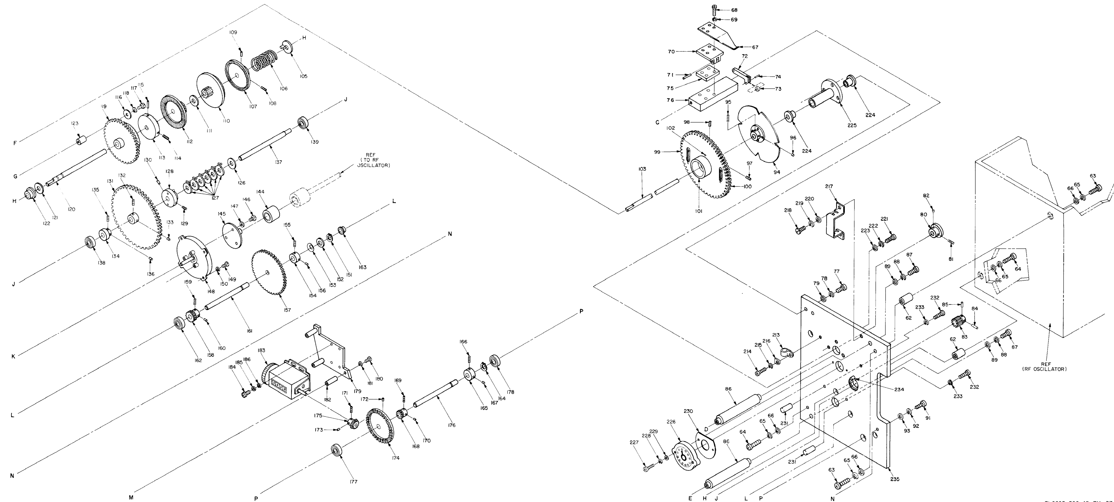
Figure 6-9 (2). Gear train, exploded view (part 2 of 2).
