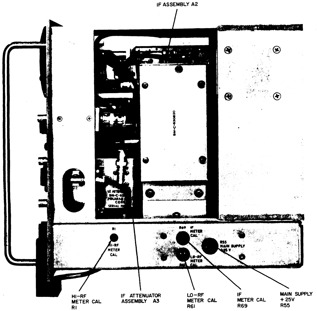
Figure 2-4. Generator, Signal SG-297/U, right side view.
