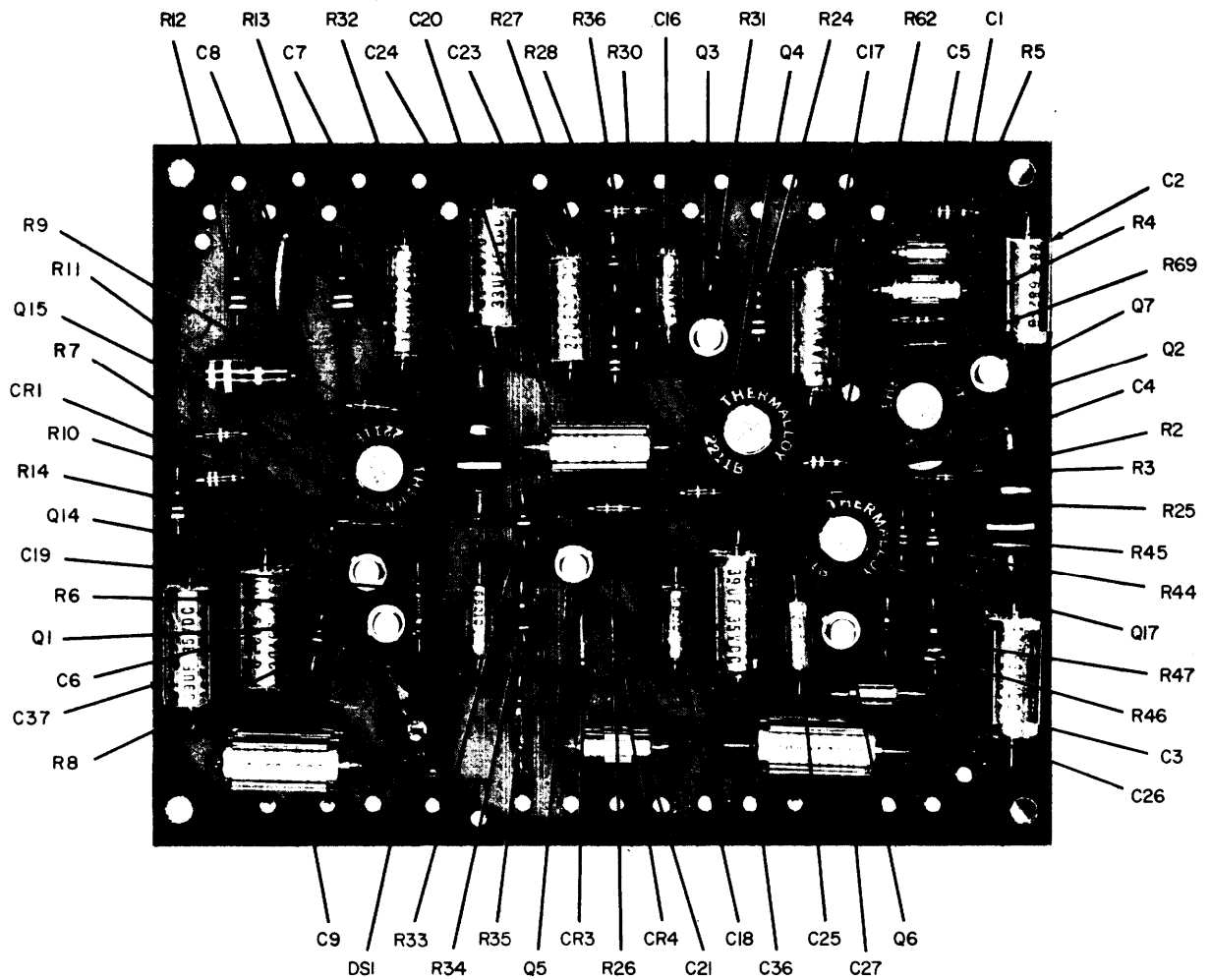
Figure 2-6. Audio board.
