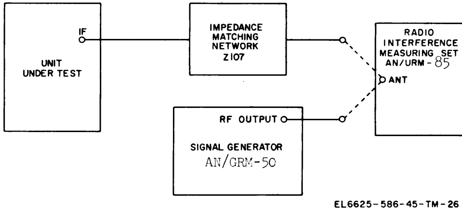
Figure 5-3. IF output level (10 UV), test setup.
