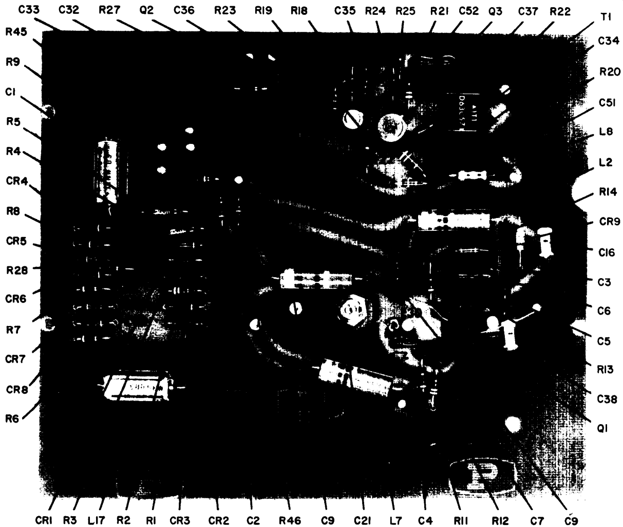
Figure 2-11. Board A1A1.
