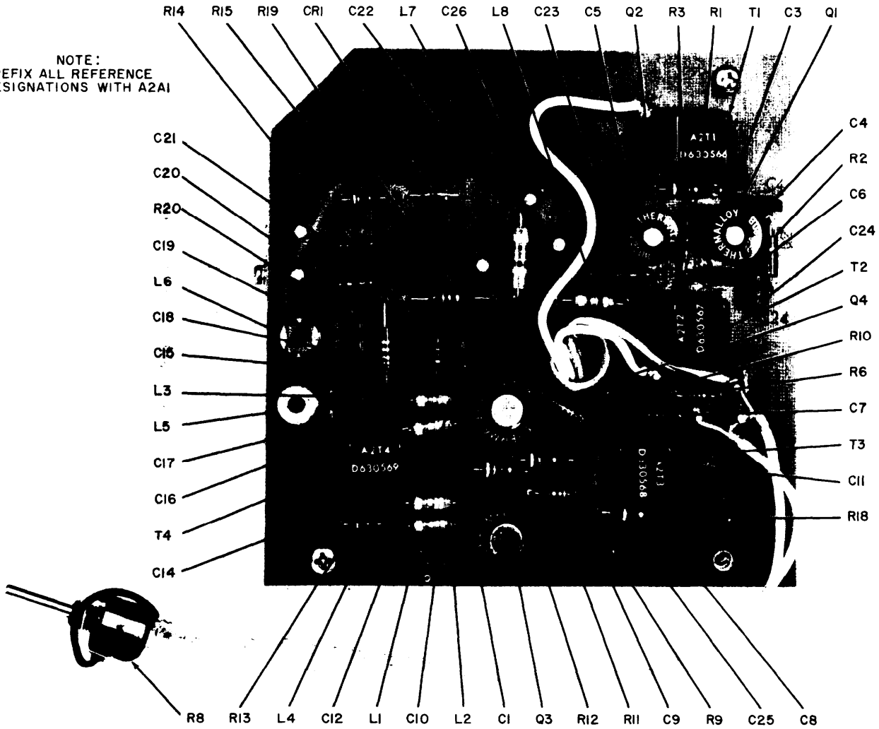
Figure 2-15. Board A2A1.
