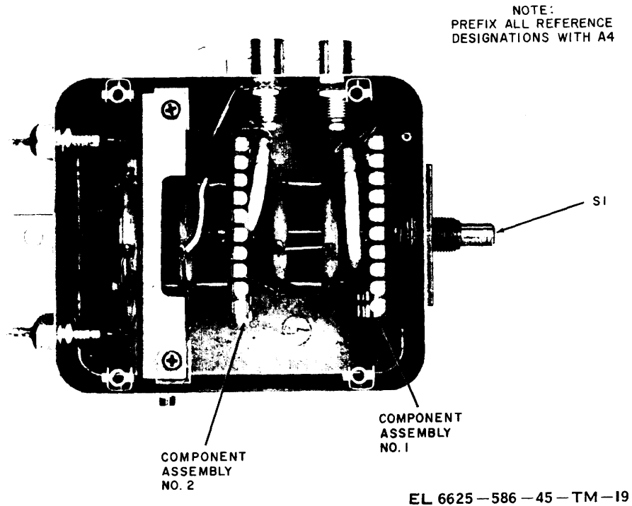
Figure 2-18. RF attenuator assembly A4, cover removed.
