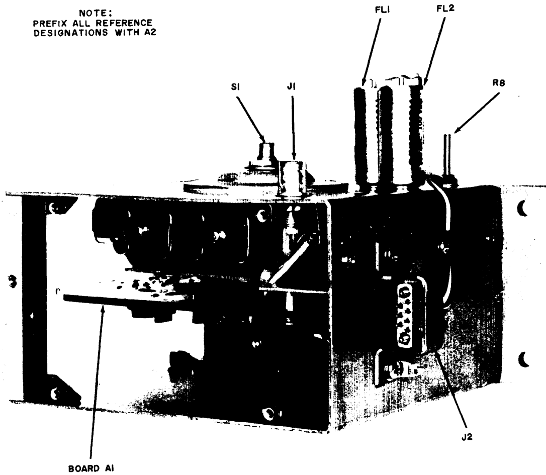
Figure 2-13. IF assembly A2, side view.
