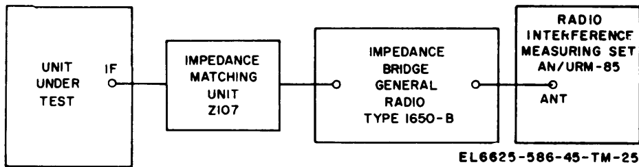
Figure 5-2. IF output impedance, test setup.
