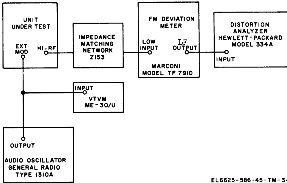
Figure 6-3. External modulation check, test connections.
